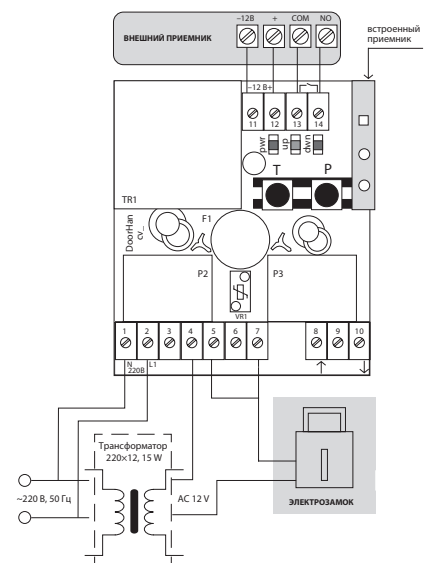
Fig. 4 Electric lock control connection diagram
